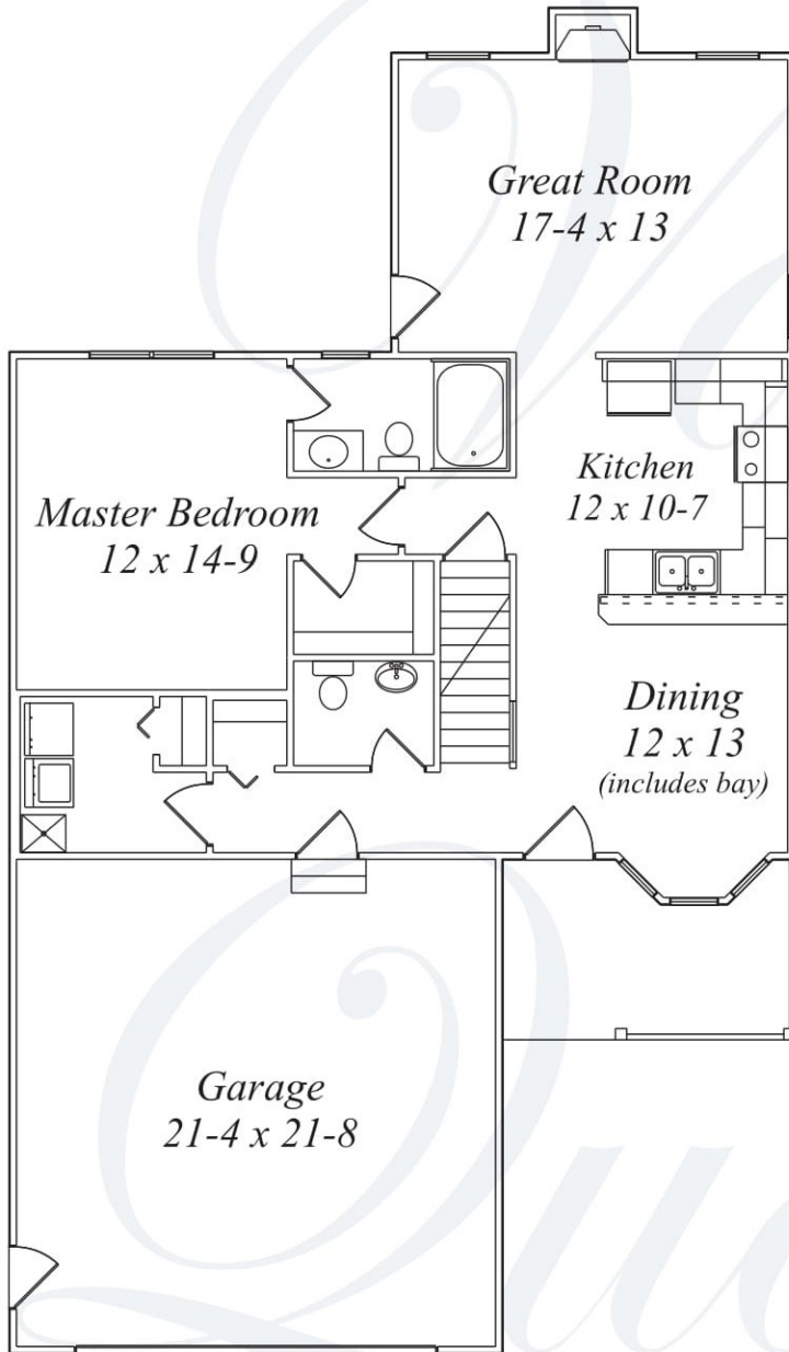
First Floor Plan 1045 Square Feet
